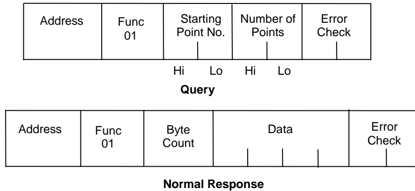
Figure 41: RTU Read Output Table Message Format
