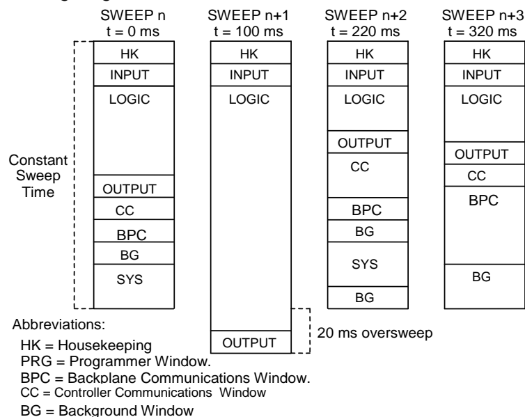
Figure 31: Typical Sweeps in Constant Sweep Mode
