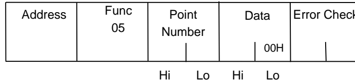
Figure 45: RTU Force Single Output Message Format
