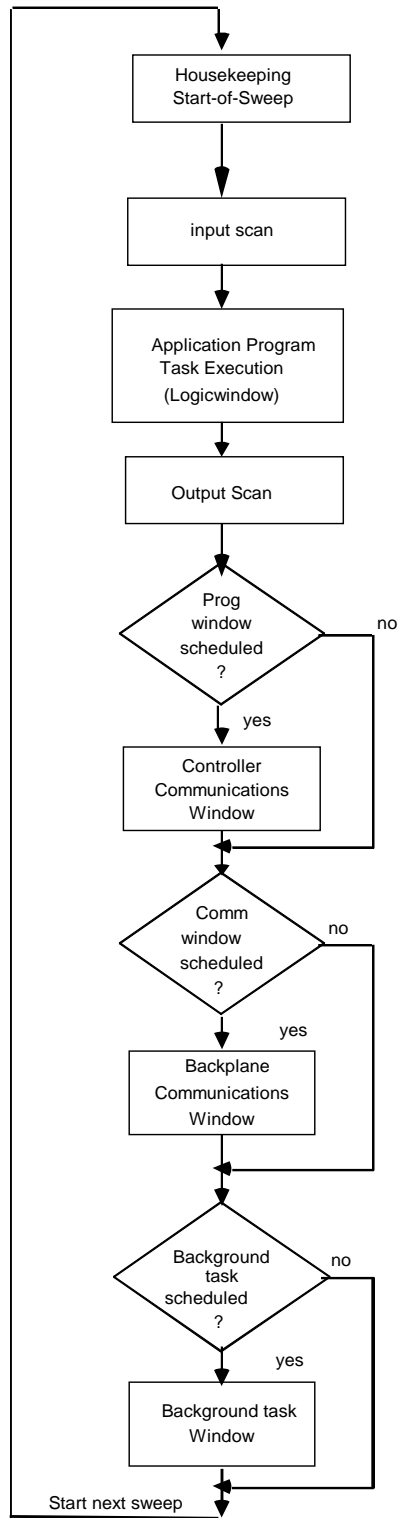
Figure 29: Major Phases of a Typical CPU Sweep
