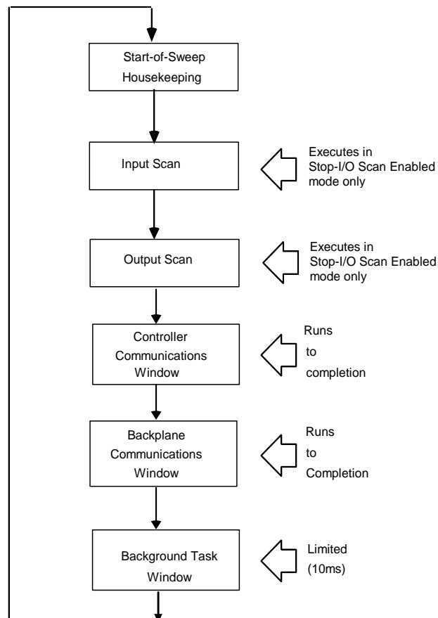
Figure 33: CPU Sweep in Stop-I/O Disabled and Stop-I/O Enabled Modes
