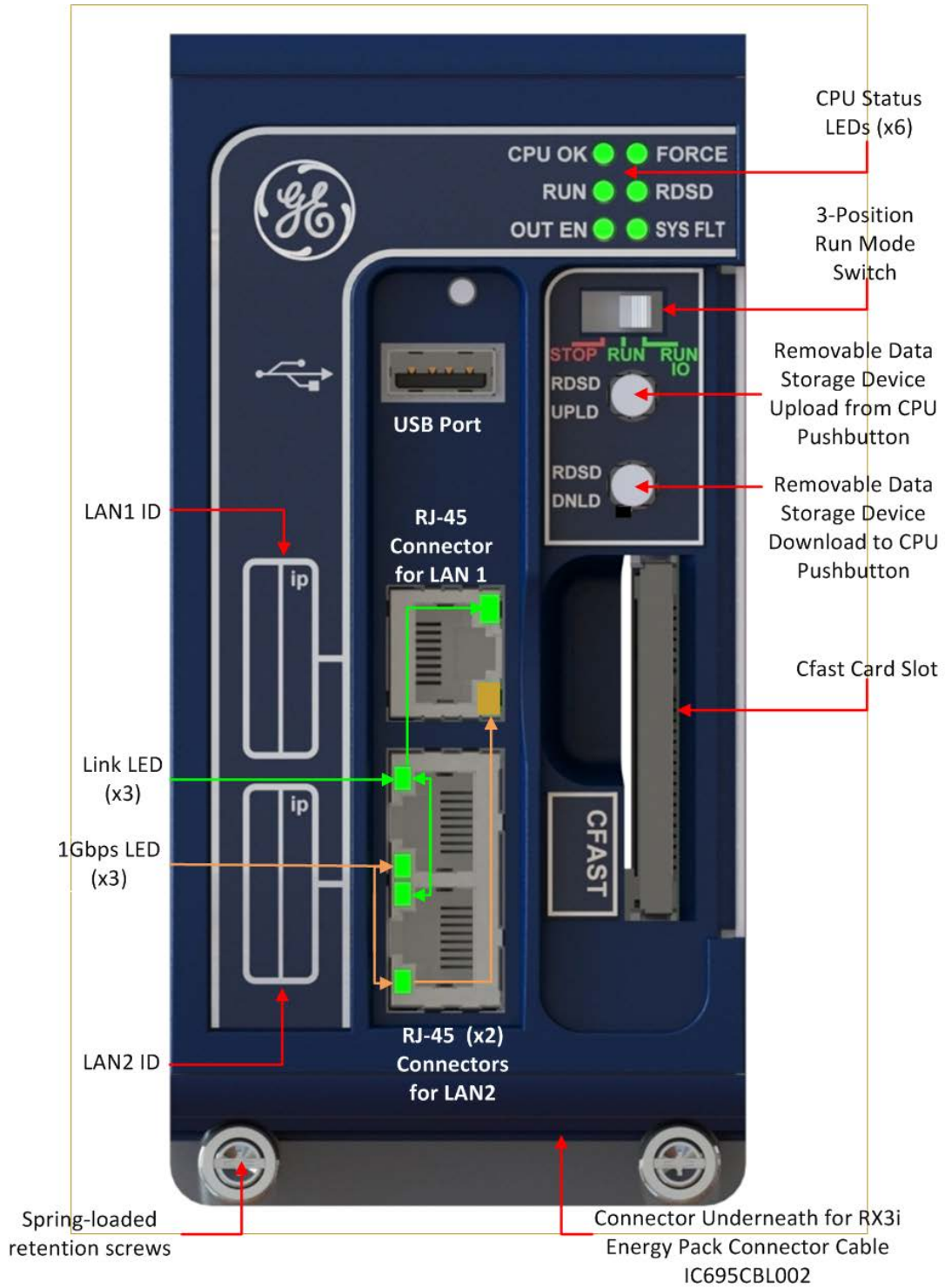
Figure 10: CPE330 Front View & Features
