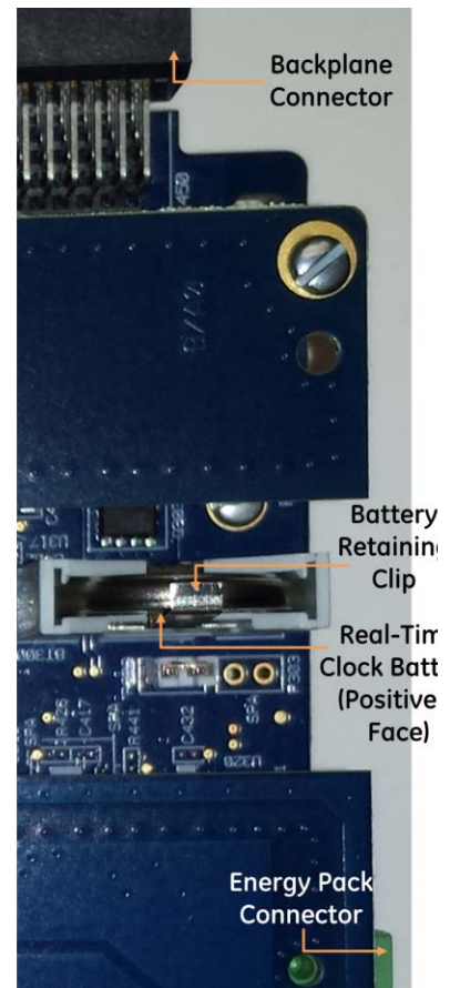
Figure 12: Location and Orientation of Real-Time Clock Battery in CPE330
