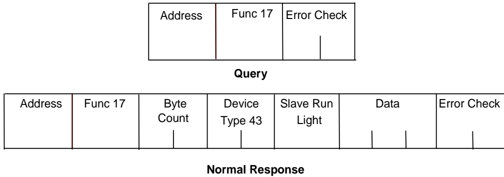
Figure 51: RTU Report Device Type Message Format
