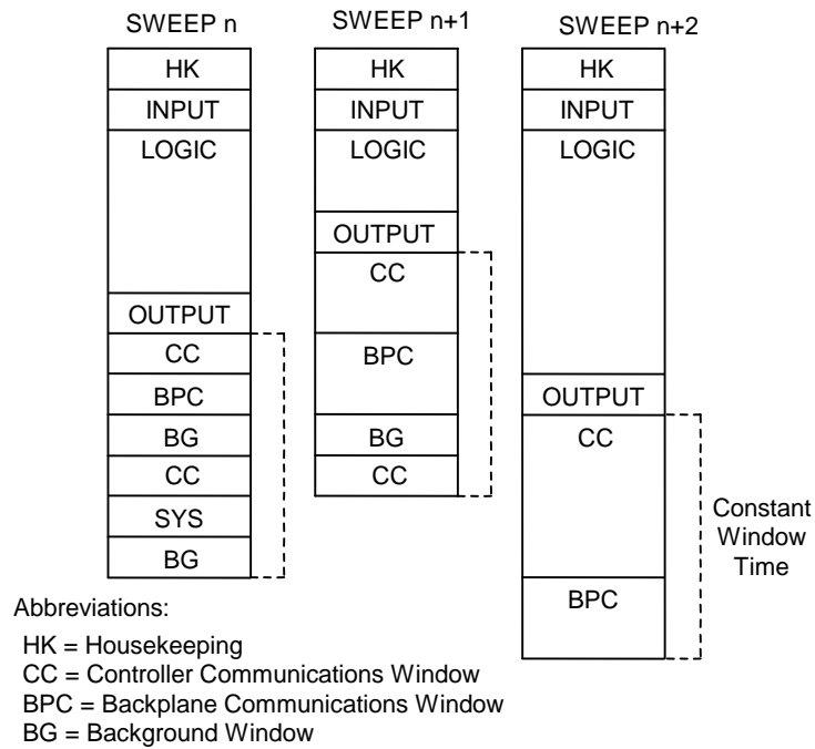
Figure 32: Typical Sweeps in Constant Window Mode
