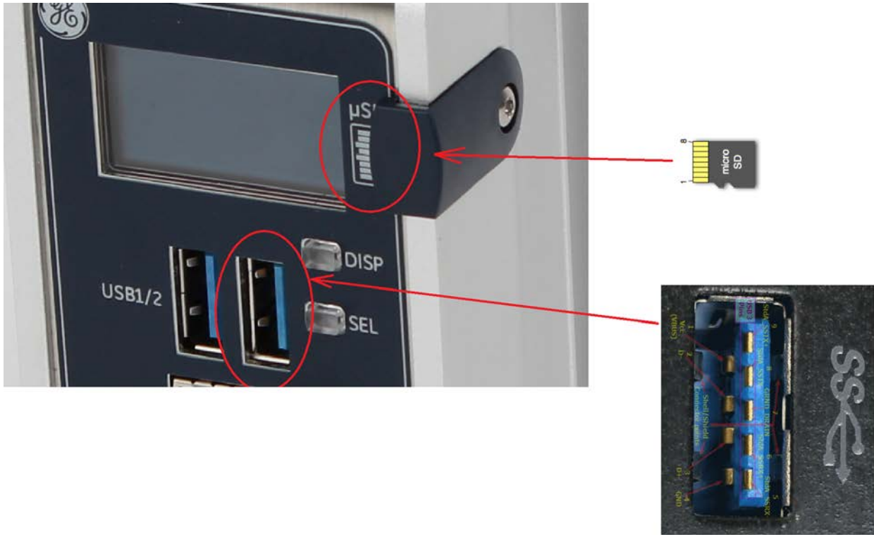
Figure 4: CPE400 Micro-SD & USB Pinouts
