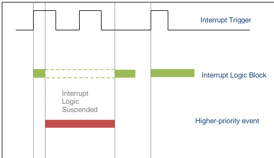
Figure 54: Interrupt Execution Considerations
