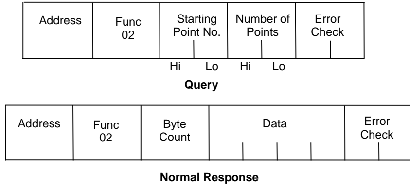
Figure 42: RTU Read Input Table Message Format
