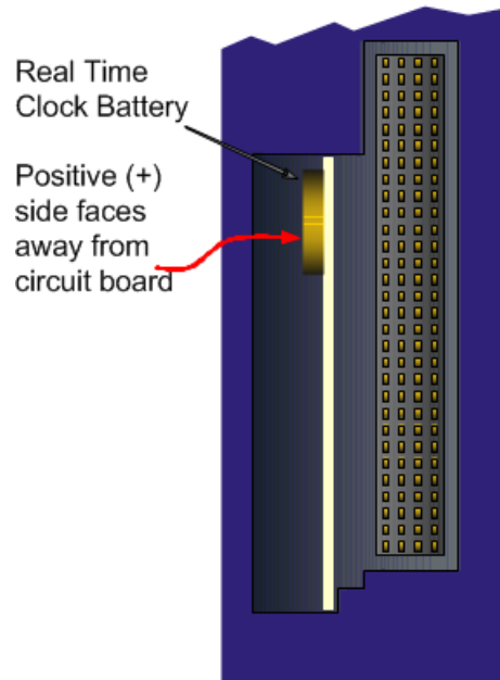
Figure 17: Accessing Real-Time Clock Battery (CPE305 and CPE310)
