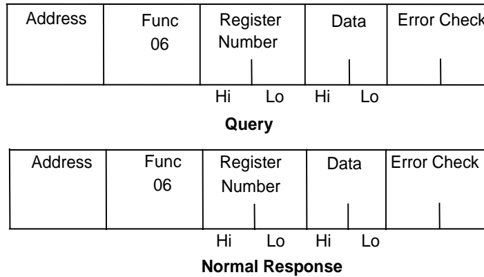
Figure 46: RTU Preset Single Register Message Format
