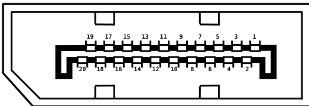
Figure 6: Display Port Connector
