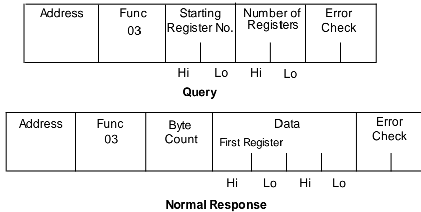
Figure 43: RTU Read Registers Message Format
