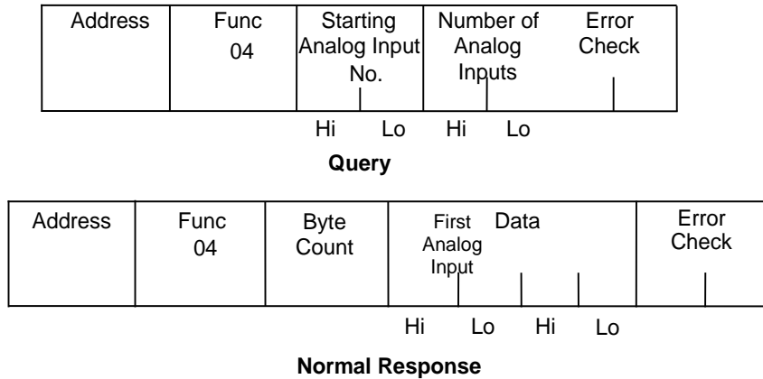
Figure 44: RTU Read Analog Inputs Message Format
