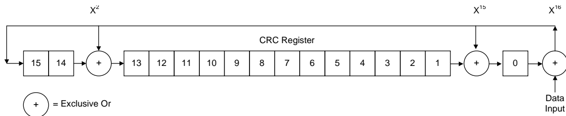
Figure 40: CRC Register Operation
