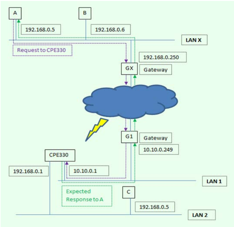
Figure 35: Expected Response Path
