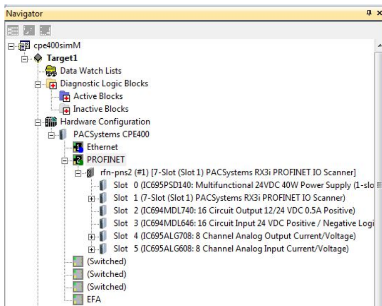
Figure 1: Configuring an Embedded PROFINET Controller
