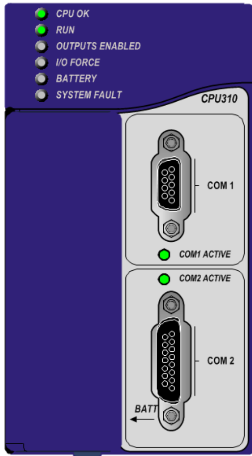
Figure 20: IC695CPU310 Front View
