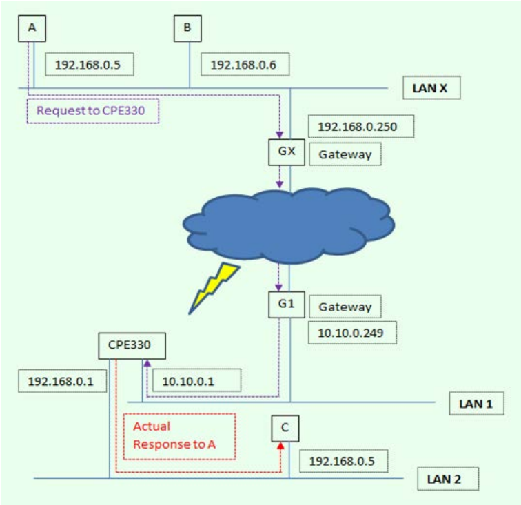
Figure 36: Actual Response Path
