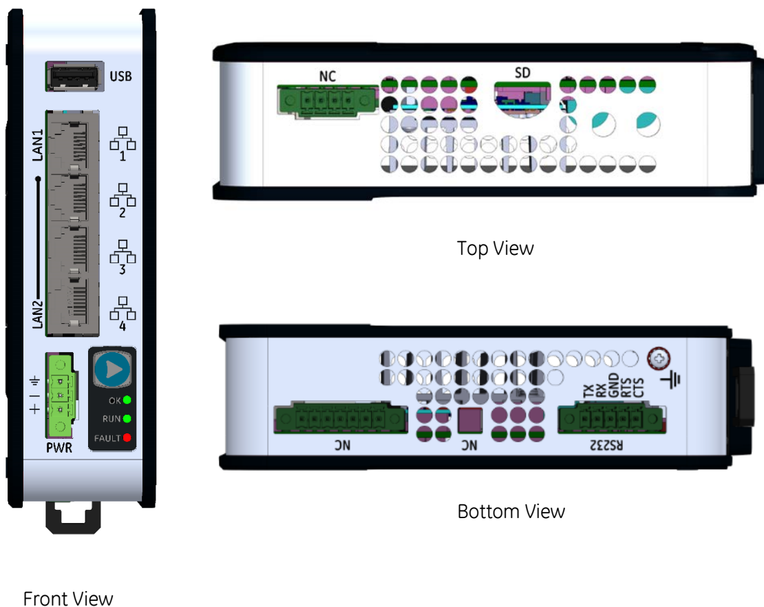
Figure 23: CPE100 Front, Top and Bottom Views of CPE100 and Features
