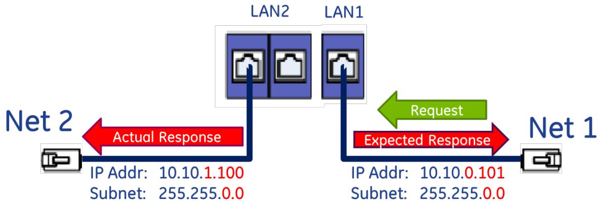
Figure 34: CPE330 Overlapping Local IP Subnet Example
