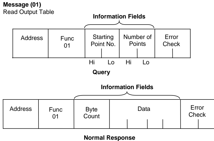
Figure 39: RTU Read Output Table Example
