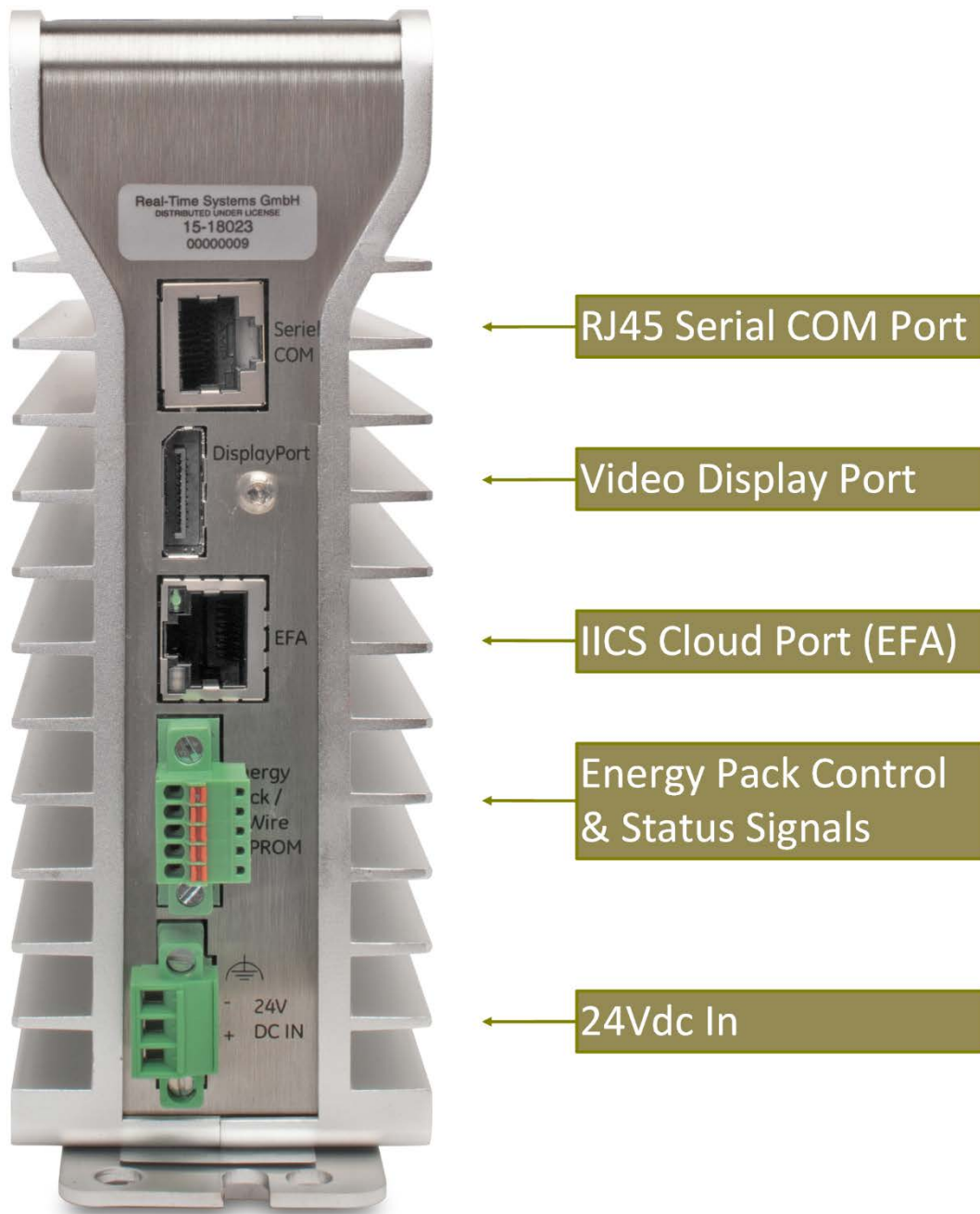
Figure 3: CPE400 Underside Ports & Connectors
