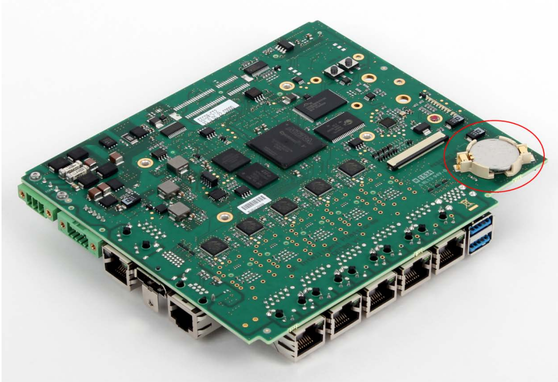
Figure 7: Location of RTC battery on CPE400
