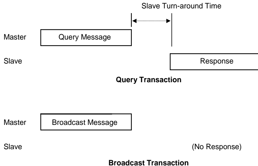
Figure 38: RTU Message Transactions
