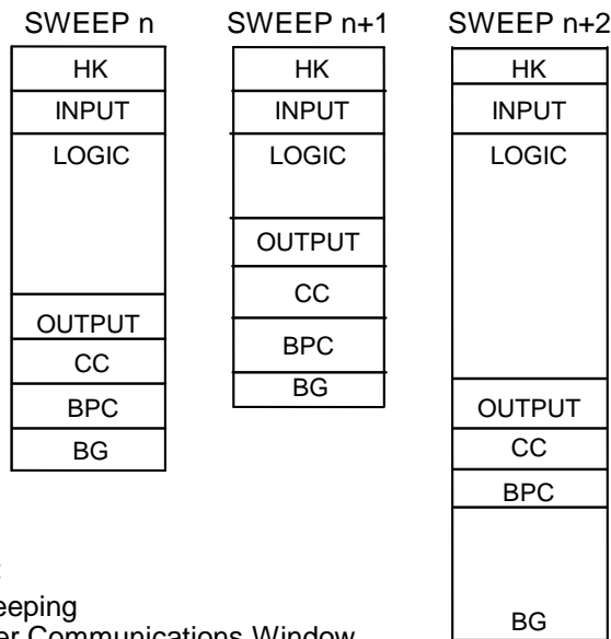
Figure 30: Typical Sweeps in Normal Sweep Mode
