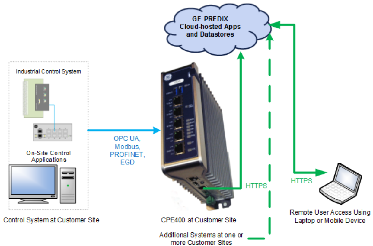
Figure 5: Typical Field Agent Application
